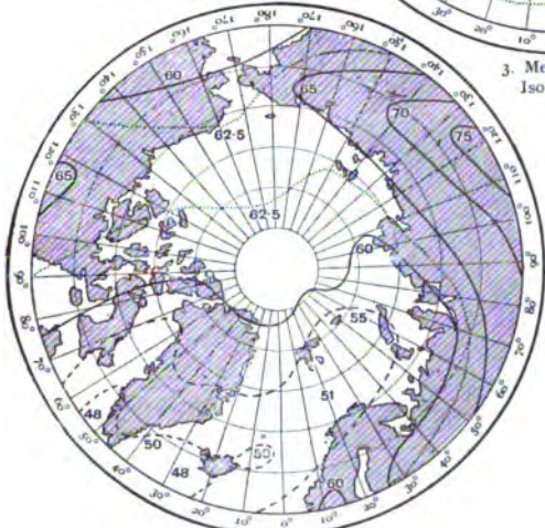
4. Isobars, January.
