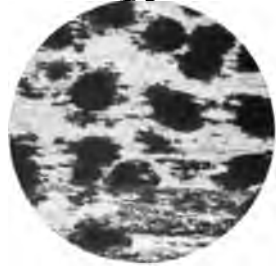
Fig. 6.—Obsidian, Iceland. In the clear glassy base there are rounded yellow spots (spherulites) arranged in fluxion streams.
