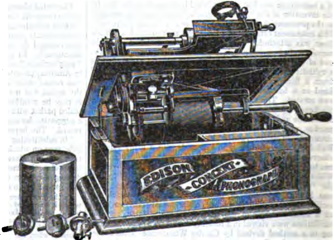
FIG. 1b.—Mechanism of Edison Phonograph.
