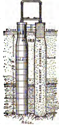
FIG. 2.—Cylindrical Piers for River Bridges.
