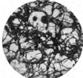
Fig. 5.—Perlitic Pitchstone, Meissen, Germany. The perlitic, rounded cracks are very clearly seen, because the rock is decomposing and becoming slightly opaque along them. At the top there is a corroded crystal of feldspar, showing cleavage, with large circular enclosures of brownish glass.
