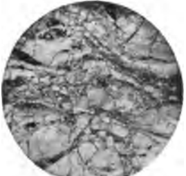
Fig. 4.—Perlitic Obsidian, Tokai, Hungary. The clear glassy rock is traversed by a large number of cracks, some long and straight, while others are nearly circular. These are rendered more distinct by the deposit of thin films of secondary limonite in them. The cracks are due to contraction on cooling.
