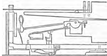
FIG. 13.—Cristofori's Escapement Action, 1720. Restored in 1875 by Cesare Fonacchi.
