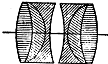
FIG. 37.—"Collinear." Series II.
