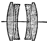
FIG. 45.—Goerz's "Color."
