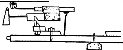
FIG. 22.—German Square Action, 1783. Piano by Wagner, Dresden.
