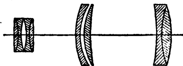
FIG. 57.—T. R. Dallmeyer's Compound Telephotographic Lens.
