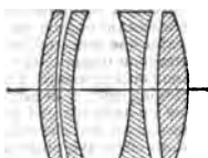
FIG. 44.—Zeiss's "Unar."
