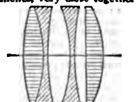
FIG. 51.—Zeiss's Tessar.
