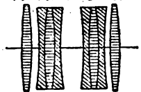
FIG. 46.—Goerz's "Alethar."
