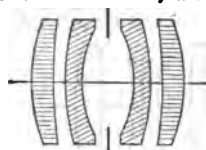
FIG. 50.—Ross's "Homocentric."
