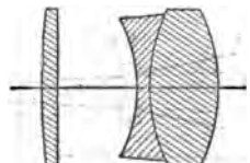
FIG. 48.—Aldis Lens. Series III.
