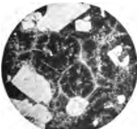
Fig. 7.—Spherulitic Rhyolite, Hlinik, Hungary. The white, angular patches are crystals of quartz and of sanidine feldspar. Between them there is a yellowish glass showing circular areas with a well-defined radiate fibrous structure (spherulites).
