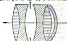
FIG. 42.—Stigmatic Lens. Series II.
