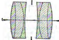
FIG. 36.—Steinheil's "Orthostigmat."
