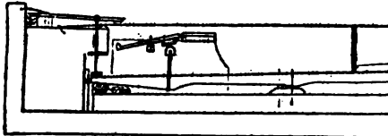
FIG. 19.—Zumpe's Square Piano Action, 1766.
