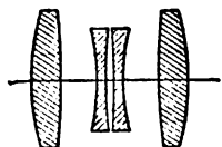
FIG. 53.—Beck-Steinheil "Unofocal."
