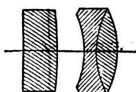
FIG. 47.—Aldis Lens. Series II.
