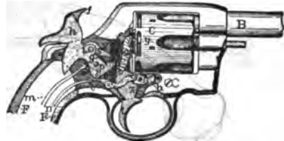
FIGS. 7 and 8.—Colt double-action revolver.
