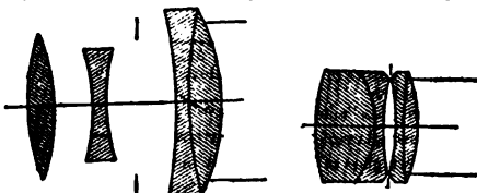
FIG. 21.—Portrait Aplanat. FIG. 22.—Group Aplanat. Form I. of 1874, but was superseded in 1881 by the "Portrait Aplanat," f/4 and free from astigmatism over an angle of 14°.
