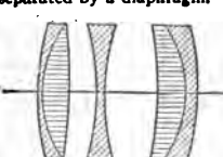
FIG. 52.—Voigtlander's Heliar.
