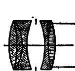
FIG. 23.—R. Steinheil's Improved Group Aplanat.
